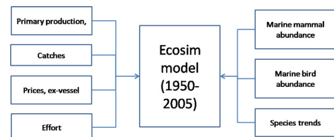
Fig. 3. Time series extraction from databases for time-dynamic Ecosim runs for each of the World's 66 LMEs.
